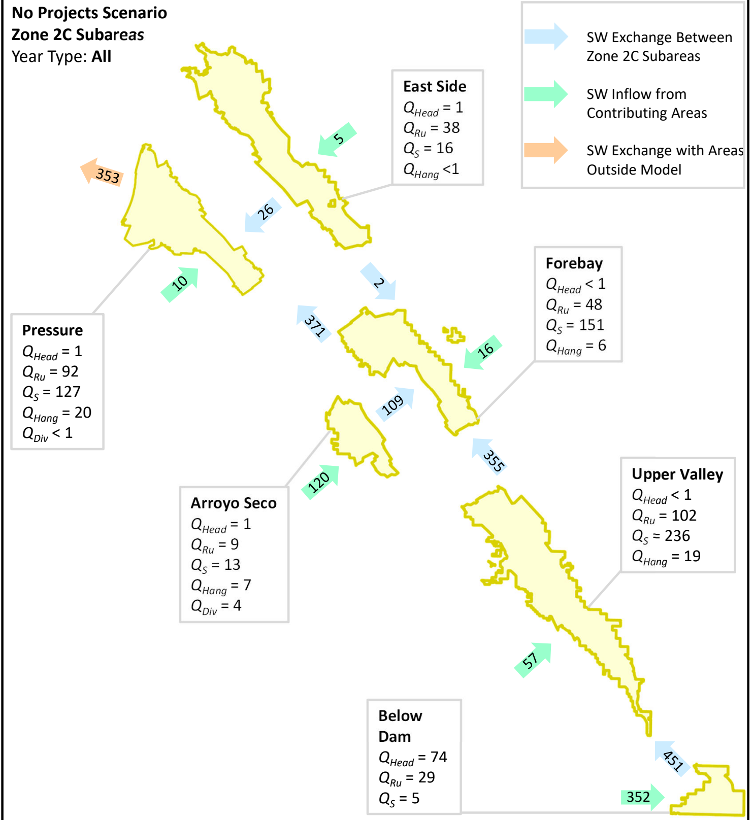
Figure 3-50 Average Annual Surface Water Budget by Subarea, No Projects Scenario
