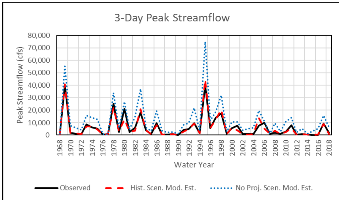
Figure B-12. Peak 3-Day Streamflow (in cfs) for Observed, Historical Scenario Modified Estimated, and No Projects Scenario Modified Estimated Datasets
