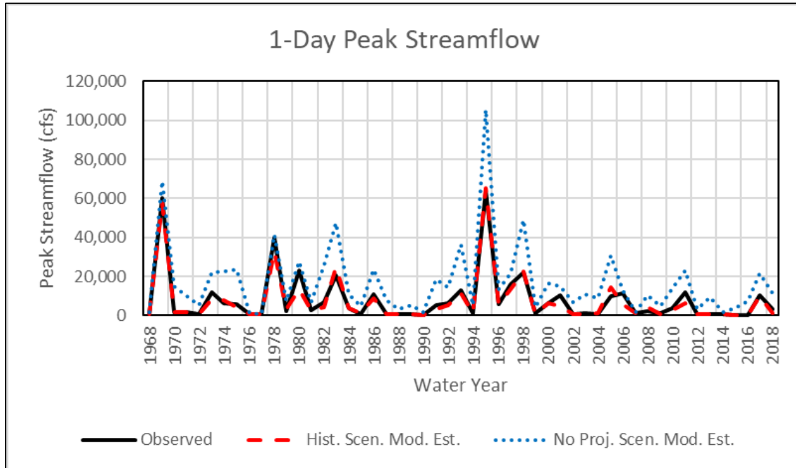
Figure B-11. Peak 1-Day Streamflow (in cfs) for Observed, Historical Scenario Modified Estimated, and No Projects Scenario Modified Estimated Datasets
