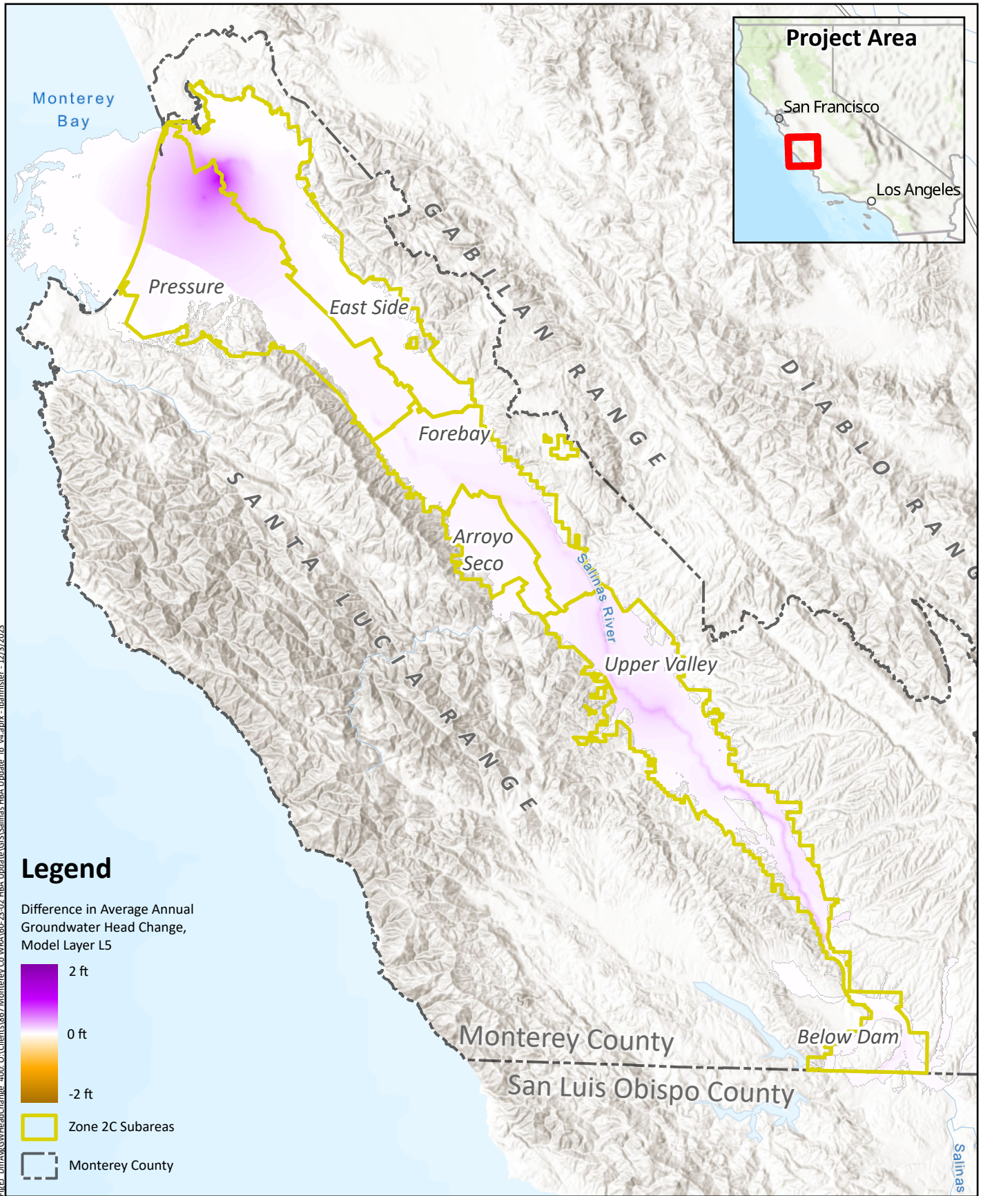
Difference in Average Annual Groundwater Head Change 400-Foot Aquifer & Equivalent
