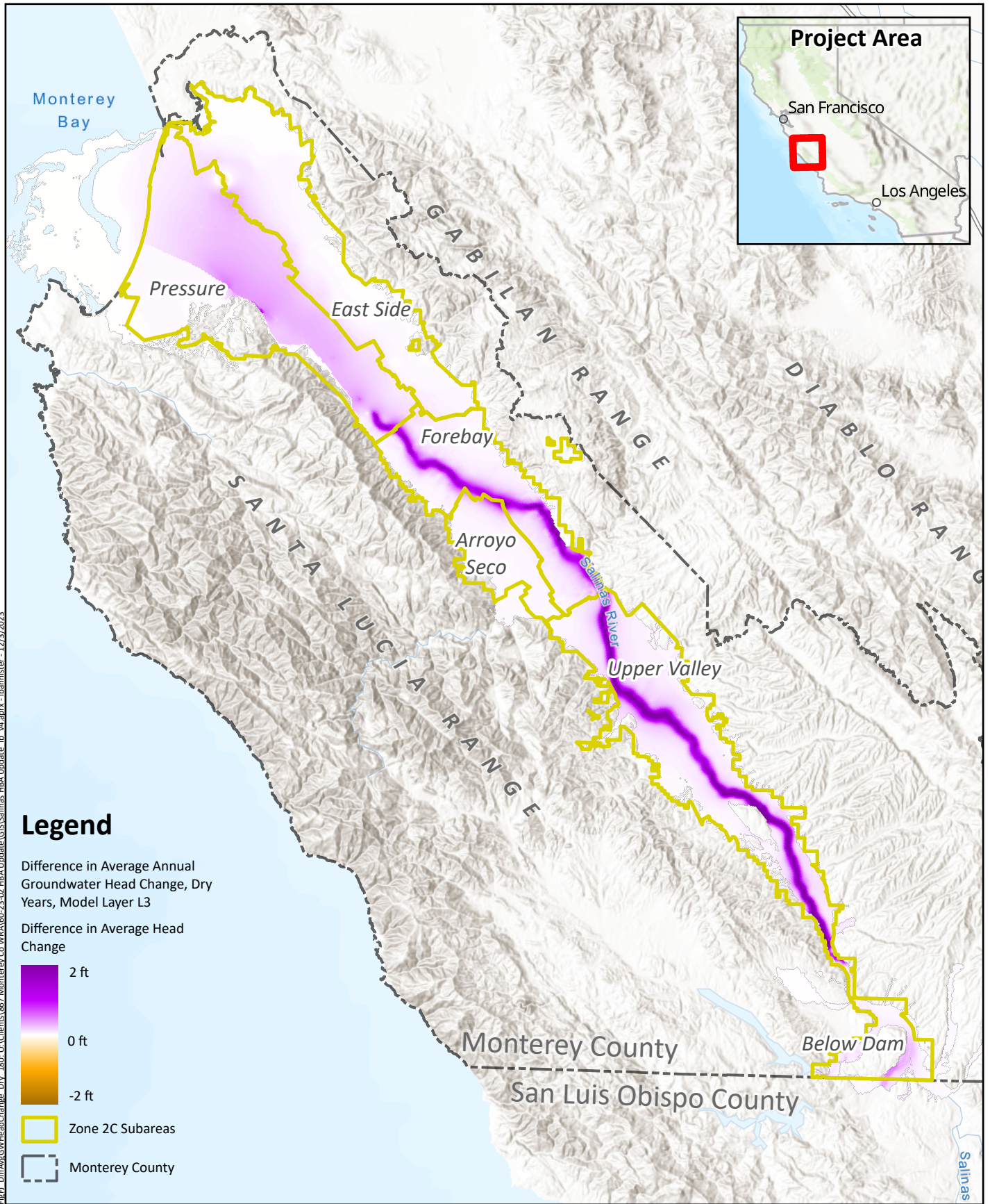
Difference in Average Annual Groundwater Head Change Dry Years 180-Footer & Equivalent
