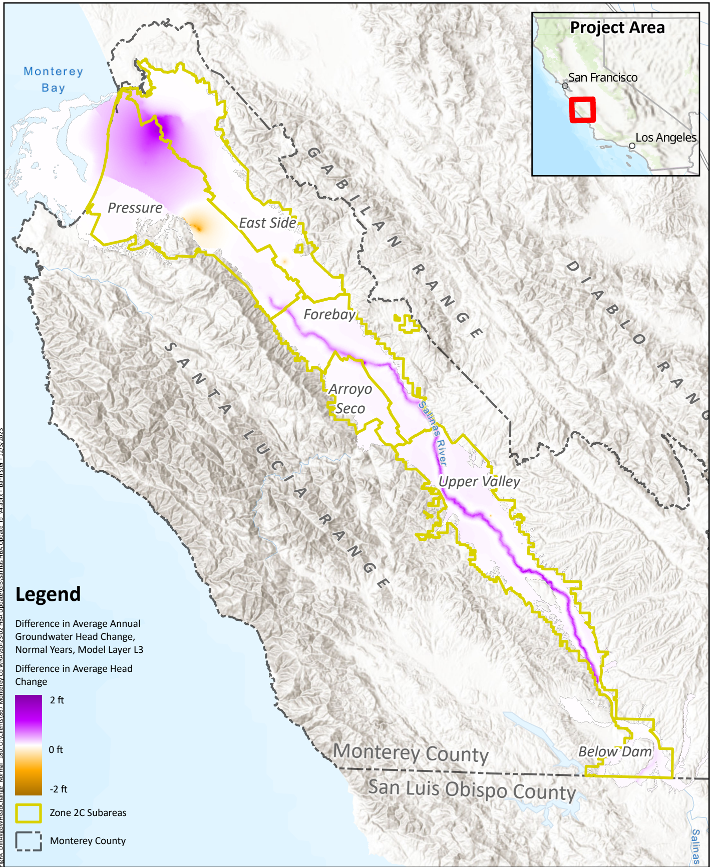
Difference in Average Annual Groundwater Head Change Normal Years 180-Footer Aquifer & Equivalent
