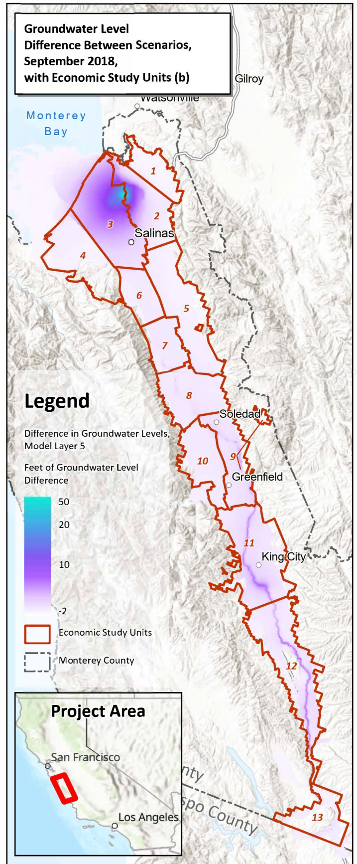
Groundwater Level Change (a) and Groundwater Level (b) Differences Between Scenarios 400-Foot Aquifer & Equivalent
