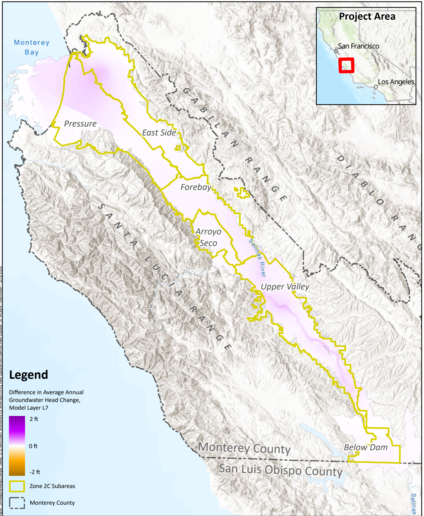
Difference in Average Annual Groundwater Head Change Deep Aquifer
