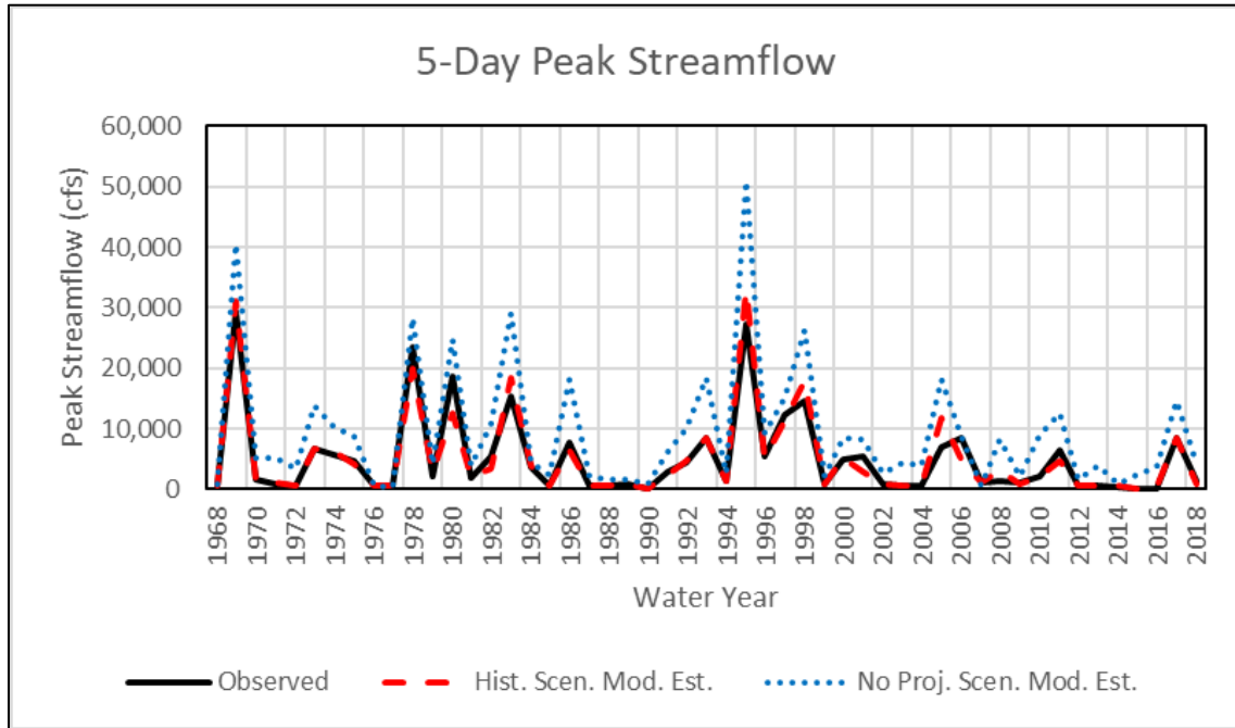
Figure B-13. Peak 5-Day Streamflow (in cfs) for Observed, Historical Scenario Modified Estimated, and No Projects Scenario Modified Estimated Datasets
