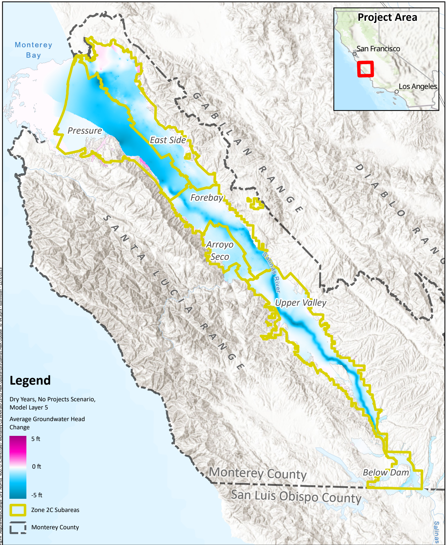
Average Annual Groundwater Head Change No Projects Scenario, Dry Years 400-Foot Aquifer & Equivalent
