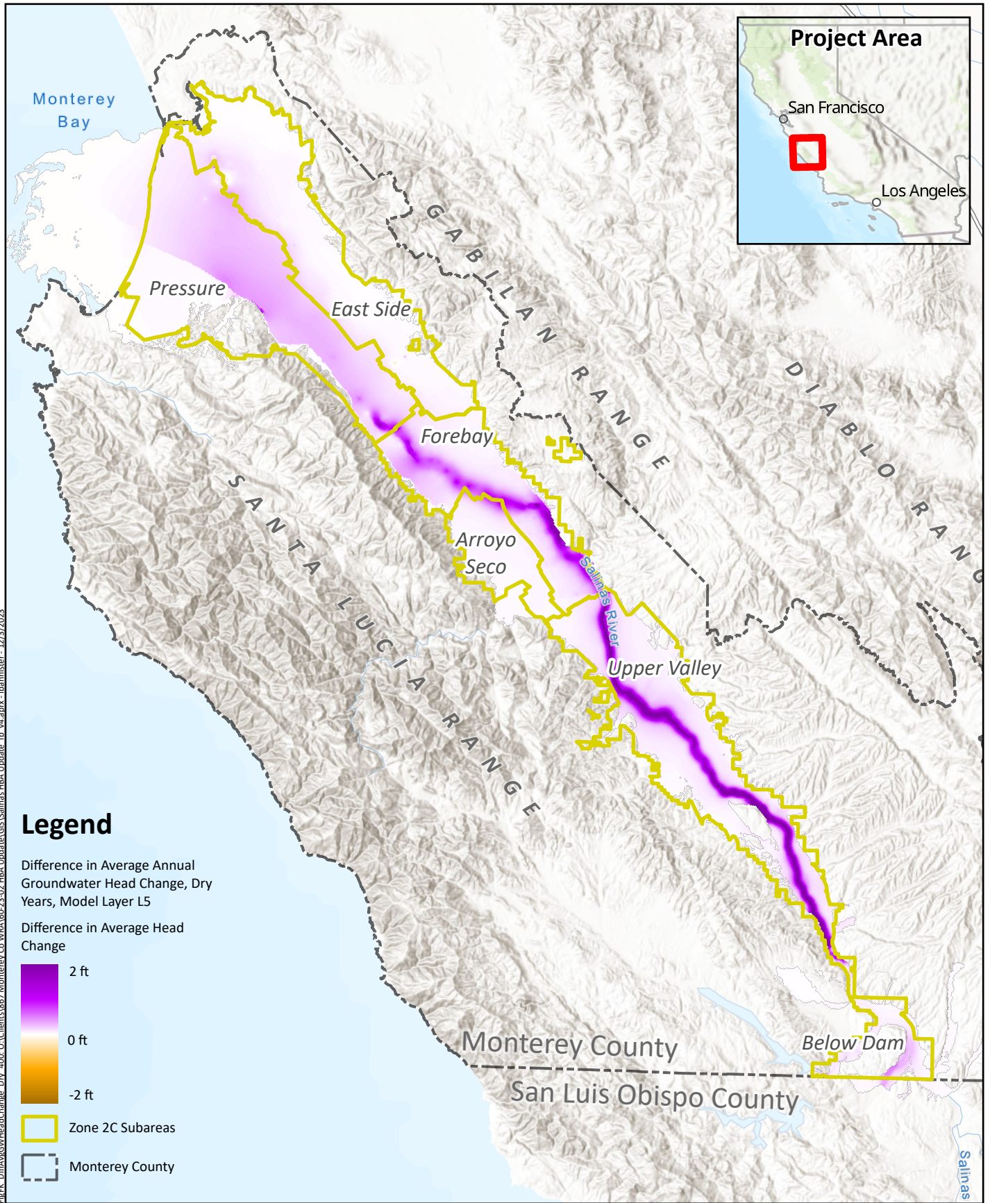
Difference in Average Annual Groundwater Head Change Dry Years 400-Footer Aquifer & Equivalent
